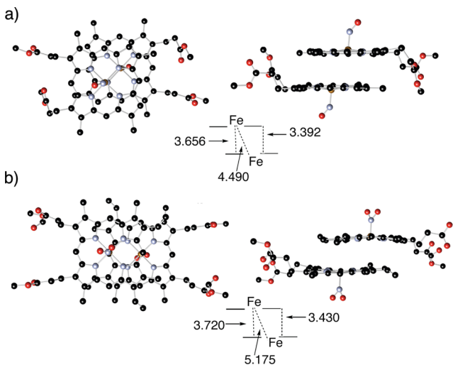
Figure 4. Diagram illustrating the solid-state interactions for (a) [Fe(DPIX-DME)(NO)] and (b) [Fe(PPIX-DME)(NO)]. Both top-down and side-on views are given.
